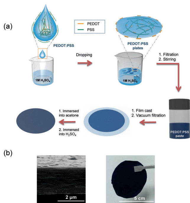
Figure 1. a) Schematic illustrations for the fabrication procedure of an HCT-PEDOT:PSS film. First, PH1000 was dropwise added into a dilute \text{H}_2\text{SO}_4 solution to obtain PEDOT:PSS plates. Then the PEDOT:PSS plates were turned into a paste by high-speed stirring. The paste was then cast onto a filter paper and the filtrate was separated by a vacuum filtration. The film was then immersed in acetone and thereafter immersed into a concentrated \text{H}_2\text{SO}_4 solution to achieve high-conductivity HCT-PEDOT:PSS films. b) Image of the free-standing HCT-PEDOT:PSS film. Cross-sectional SEM image of the HCT-PEDOT:PSS film.
