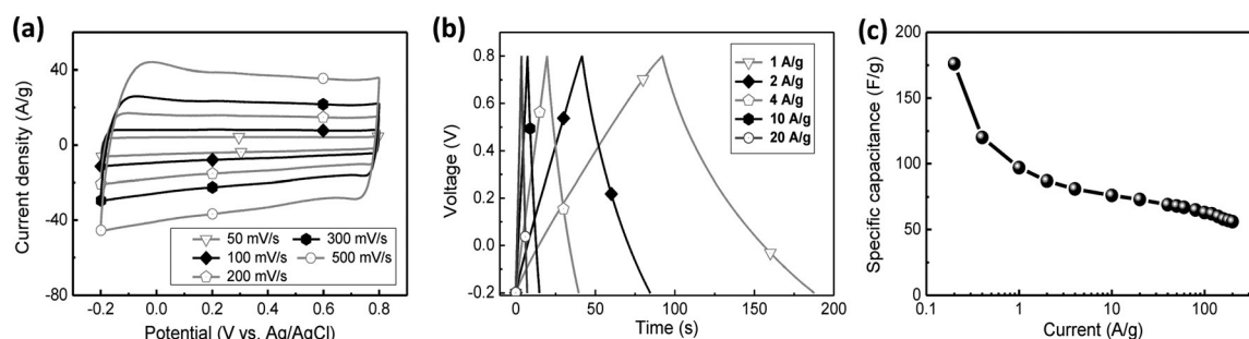
Figure 2. a) Cyclic voltammograms of HCT-PEDOT:PSS films recorded at different scan rates of 50, 100, 200, 300, and 500 \text{ mV s}^{-1} . b) Charge–discharge profiles of HCT-PEDOT:PSS films recorded at different current densities of 1, 2, 4, 10, 20 \text{ A g}^{-1} . c) The specific capacitance as a function of current density.
